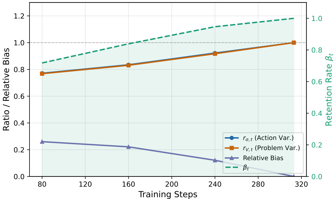
Qwen2.5-Math-1.5B (Entropy)
